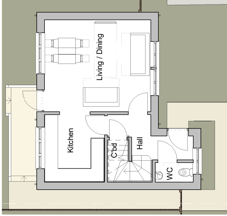
House 5 - Ground Floor Plan as Proposed 1 : 100
