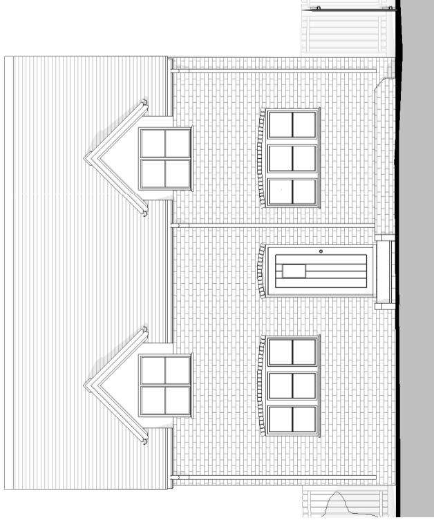
House 5 - West Elevation as Proposed 1 : 100
