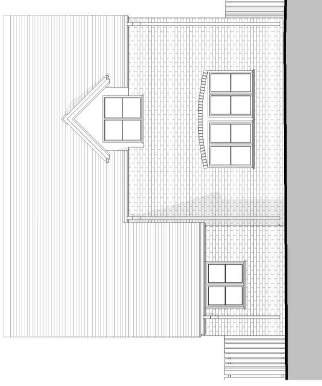
House 5 - East Elevation as Proposed 1 : 100
